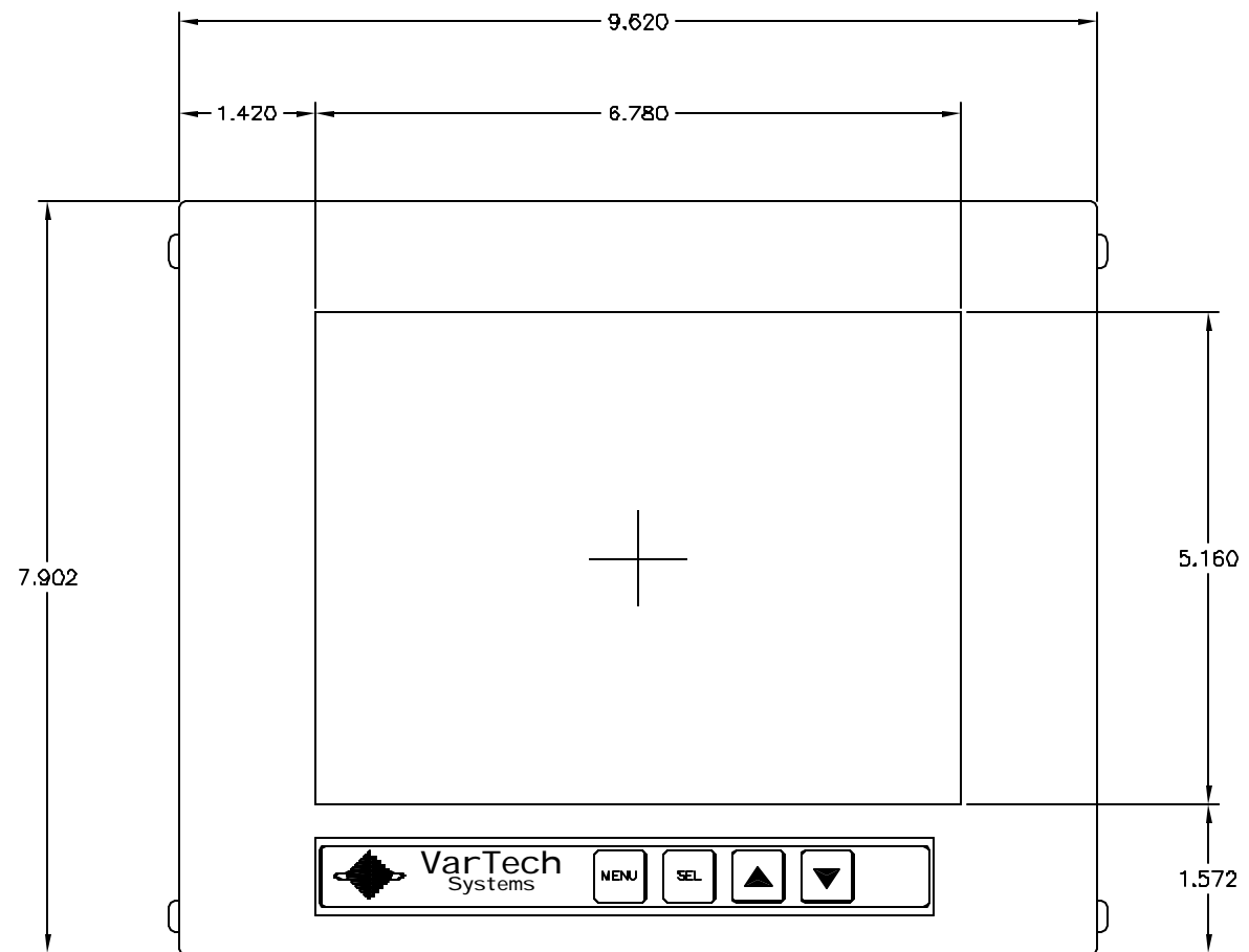
FRONT VIEW
