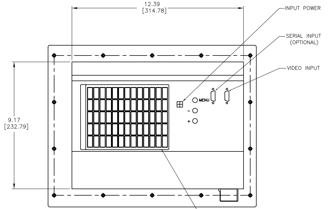
REAR VIEW
