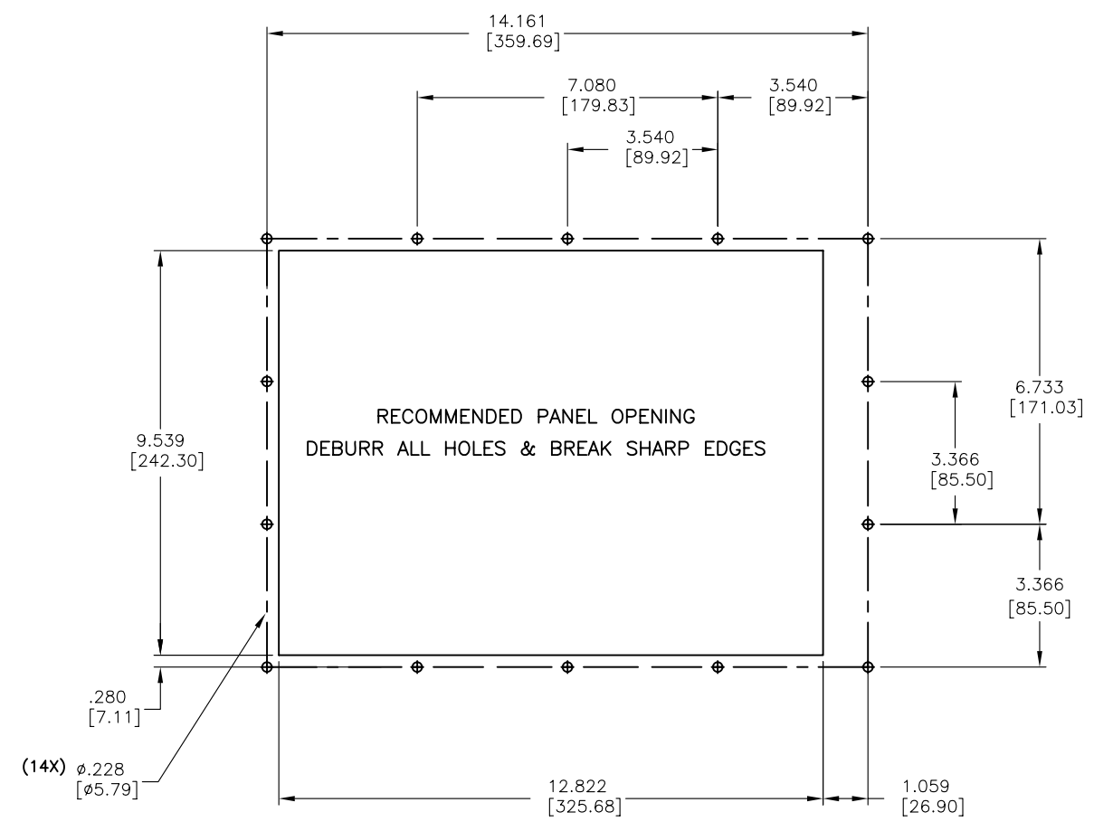
FRONT VIEW
