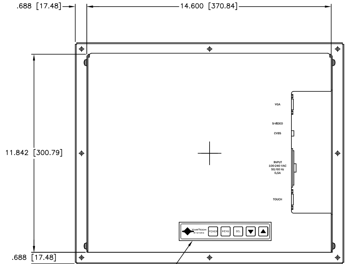
REAR CONTROLS
