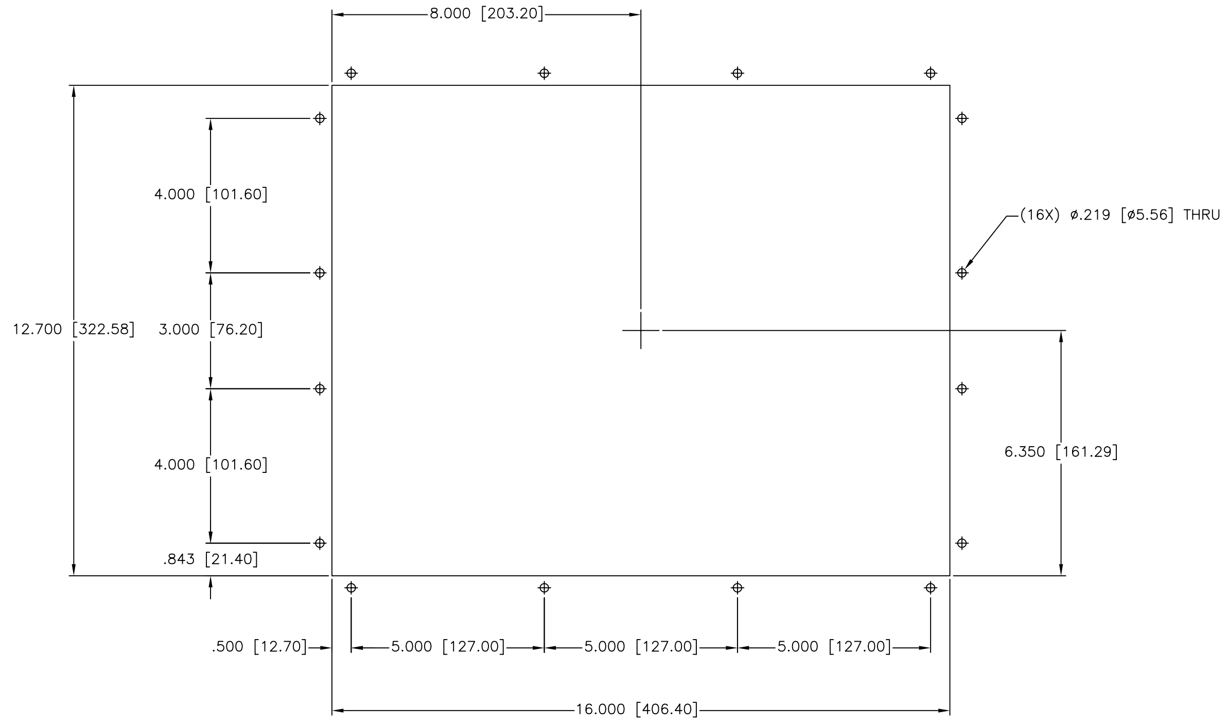
CUTOUT DETAIL
