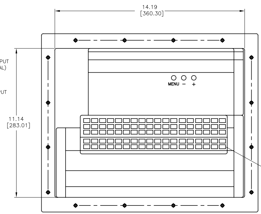
REAR VIEW
