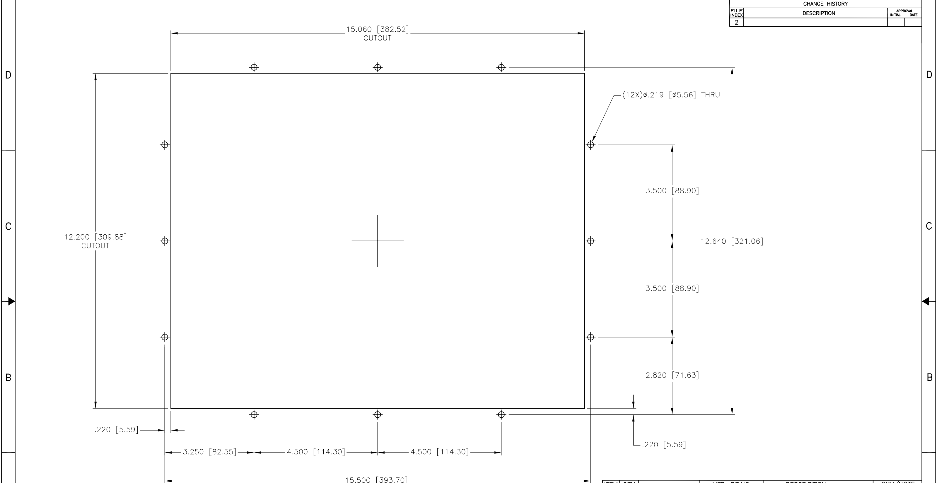
CUTOUT VIEW
