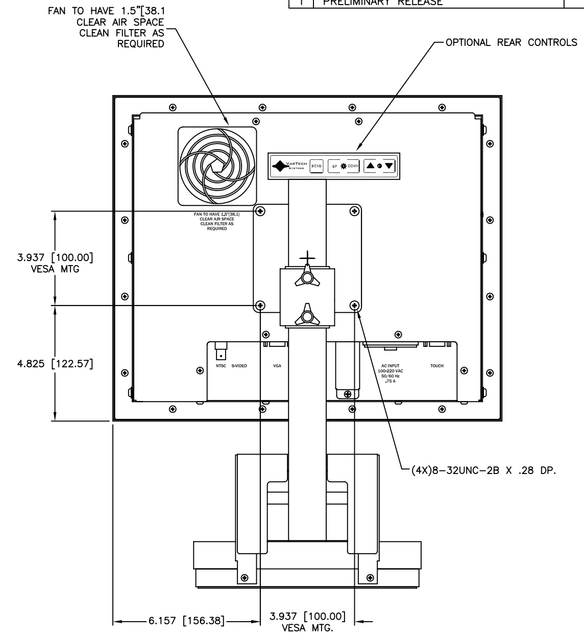
REAR VIEW
