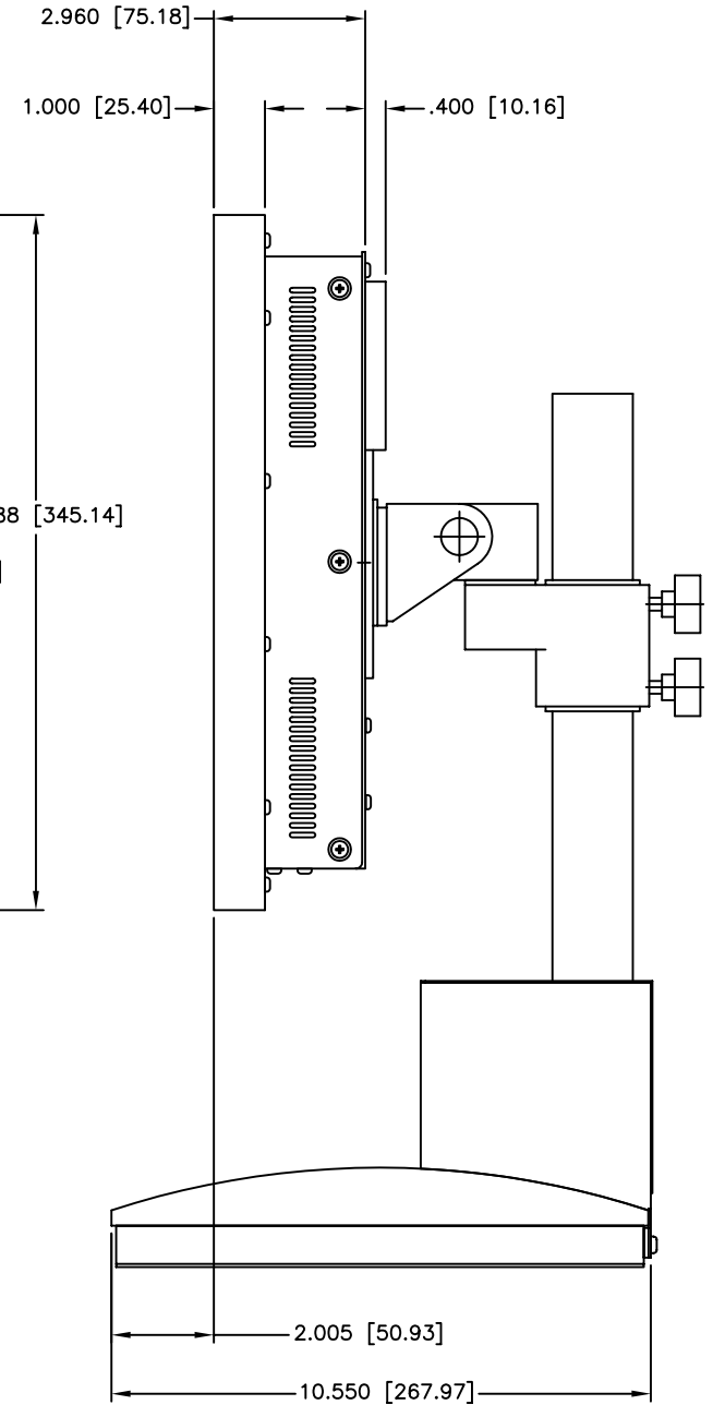
SIDE VIEW
