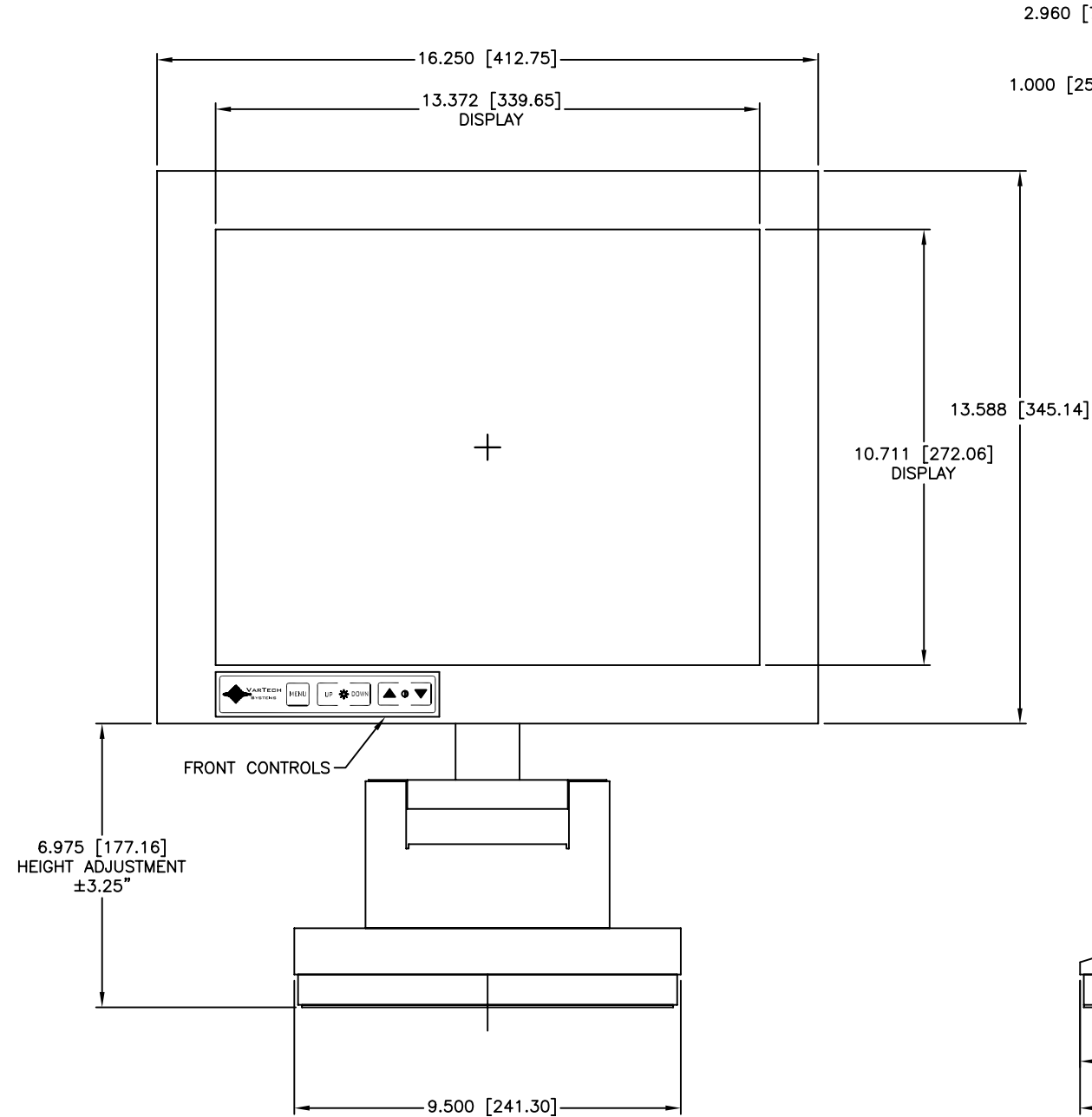
FRONT VIEW
