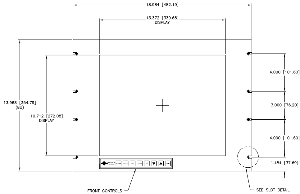
FRONT VIEW
