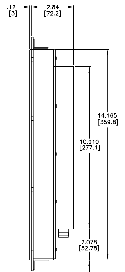
SIDE VIEW
