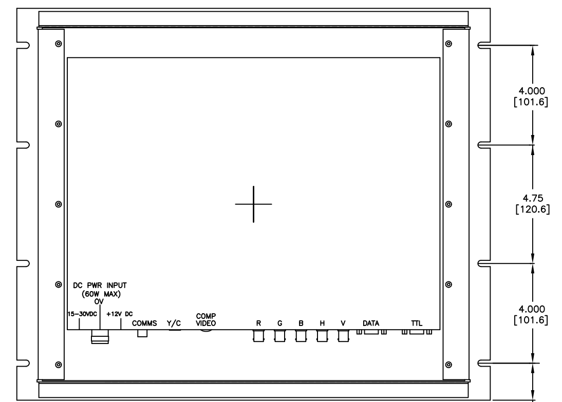
REAR VIEW
