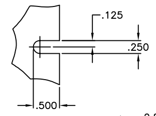
DETAIL C SCALE 2/1 8 REQ'D
