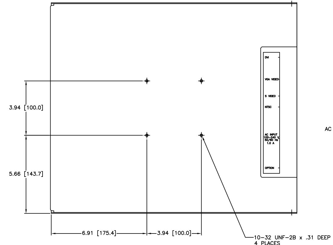
REAR VIEW
