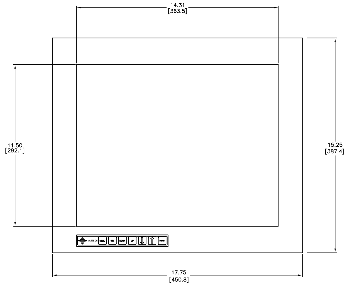
FRONT VIEW
