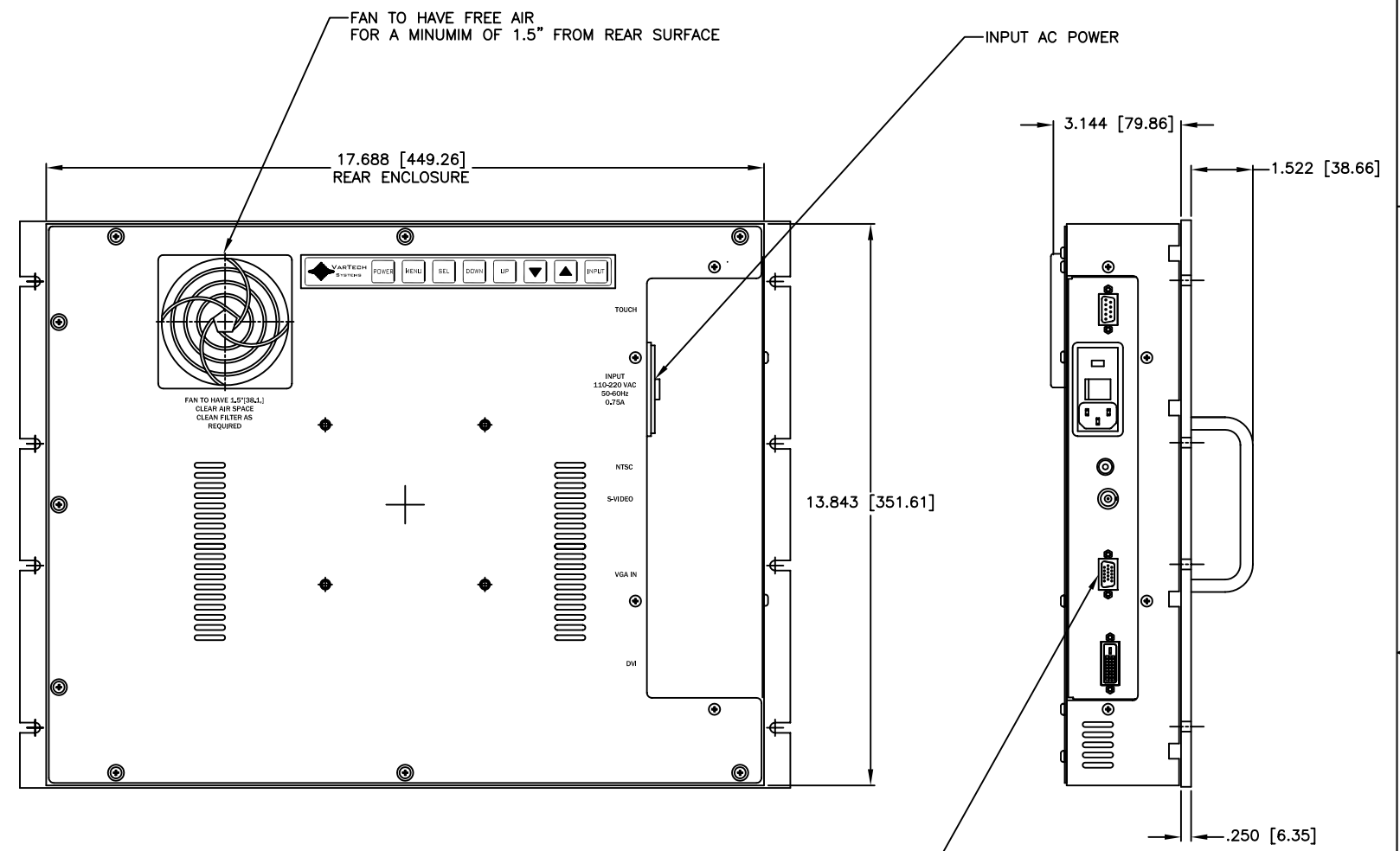
REAR PANEL CONNECTIONS
