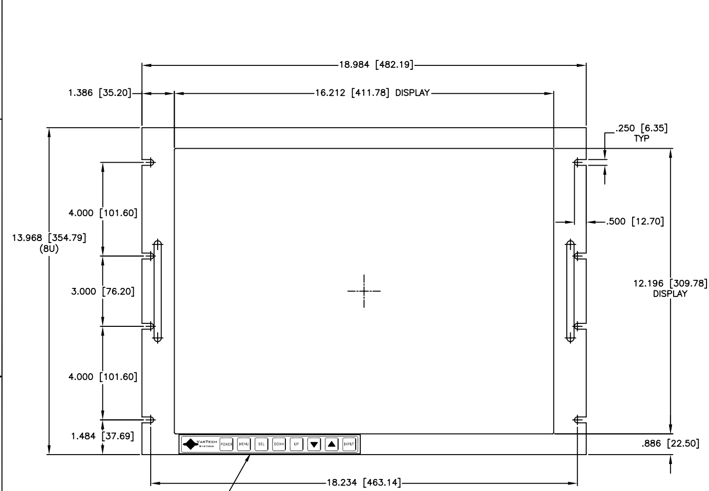
FRONT VIEW
