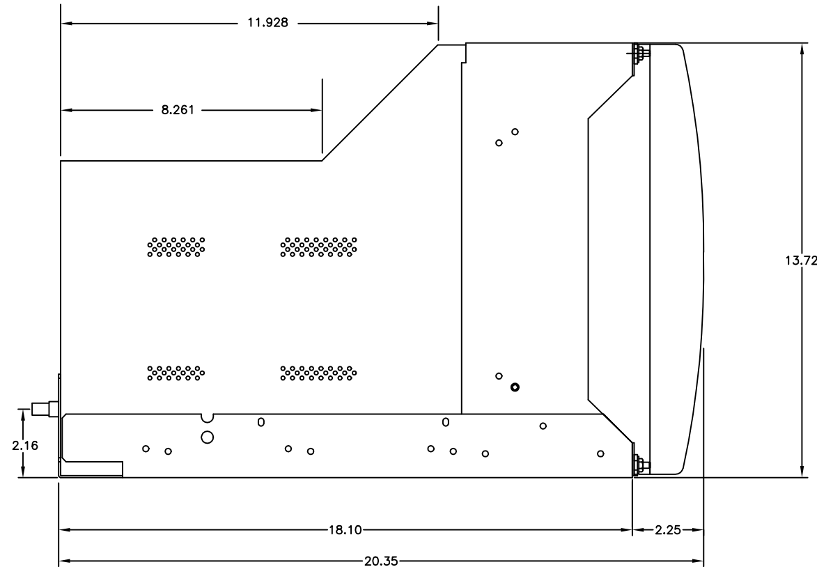
SIDE VIEW
