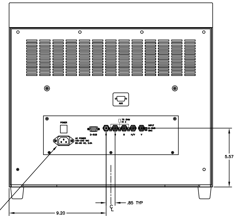
REAR VIEW
