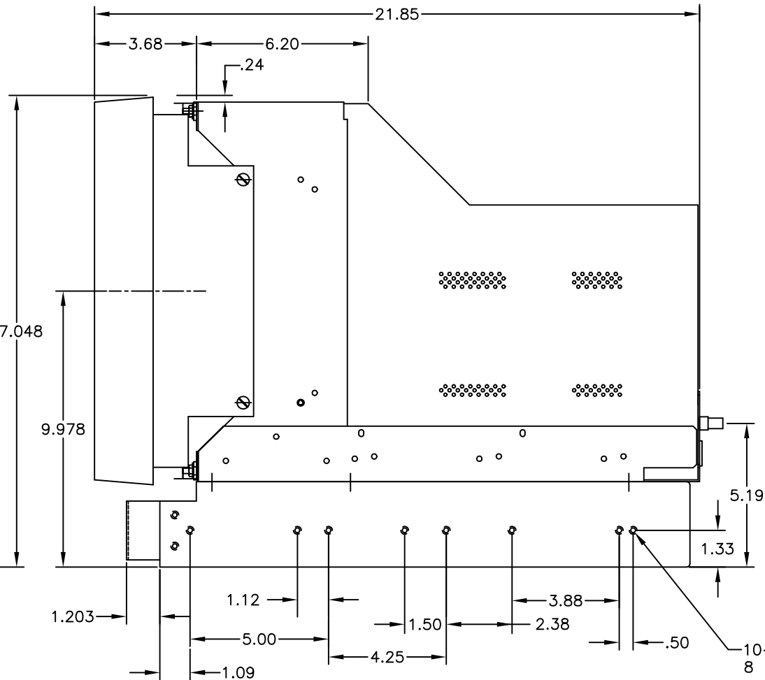
SIDE VIEW
