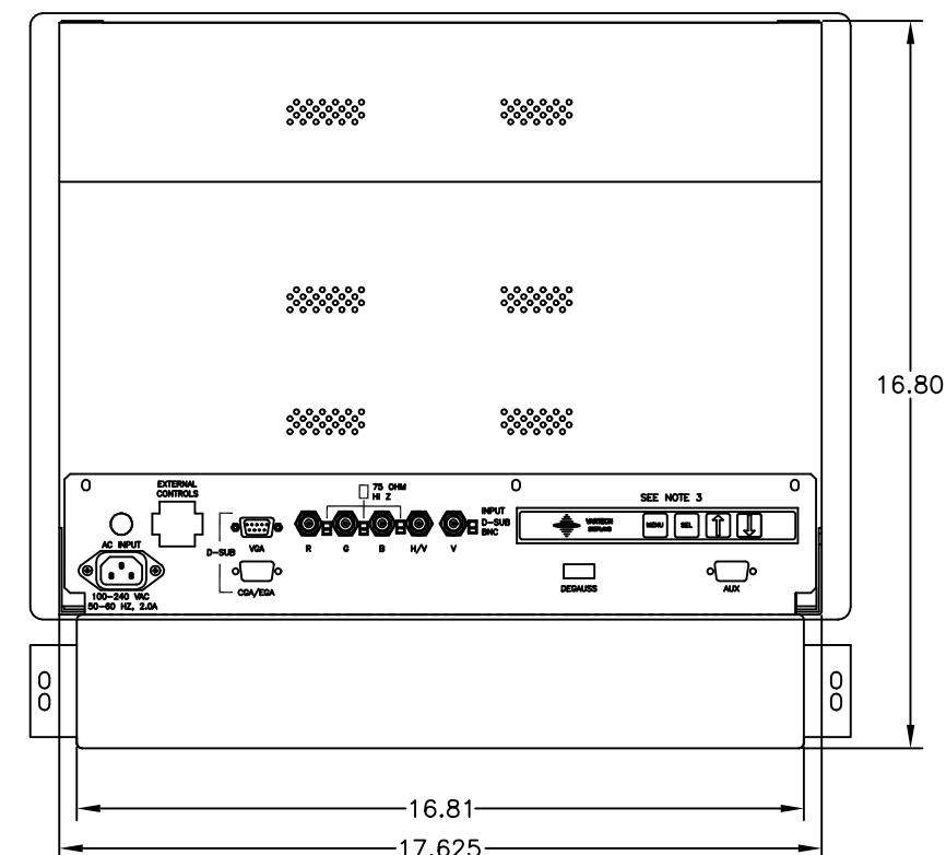
REAR VIEW
