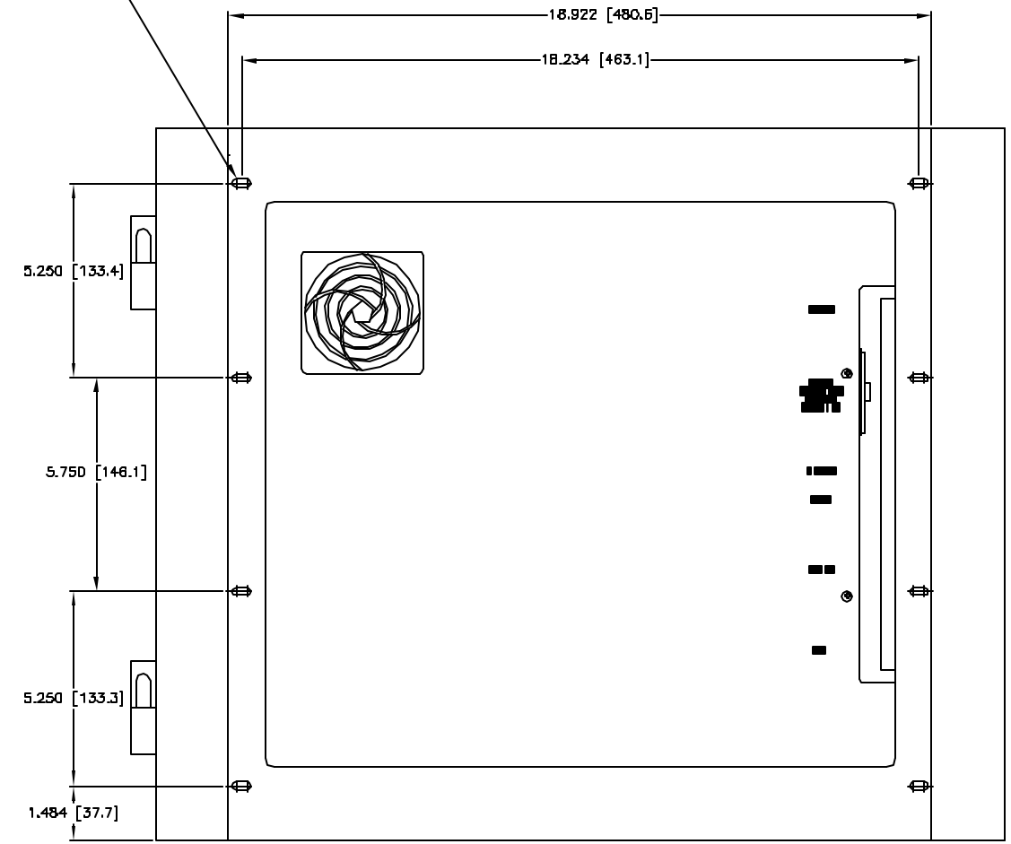
REAR VIEW
