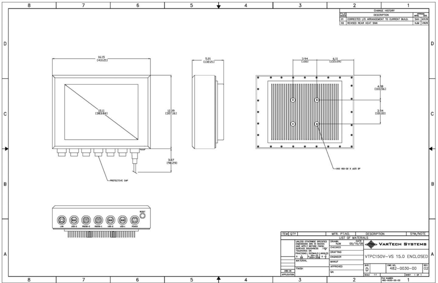
Product Drawing: Detail -A-
