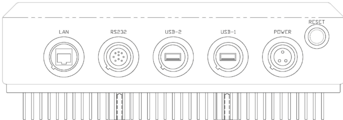
Bottom Rear View - Connector Panel -
